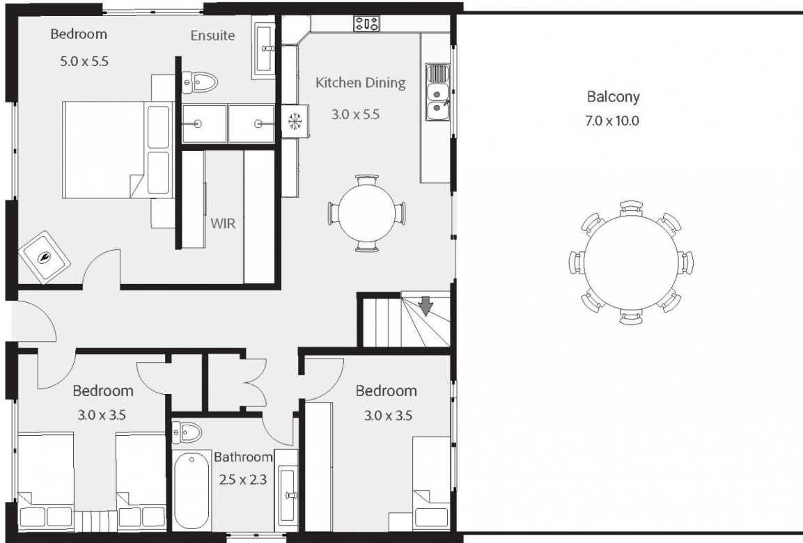
▼ Ground Floor - Upper Level
